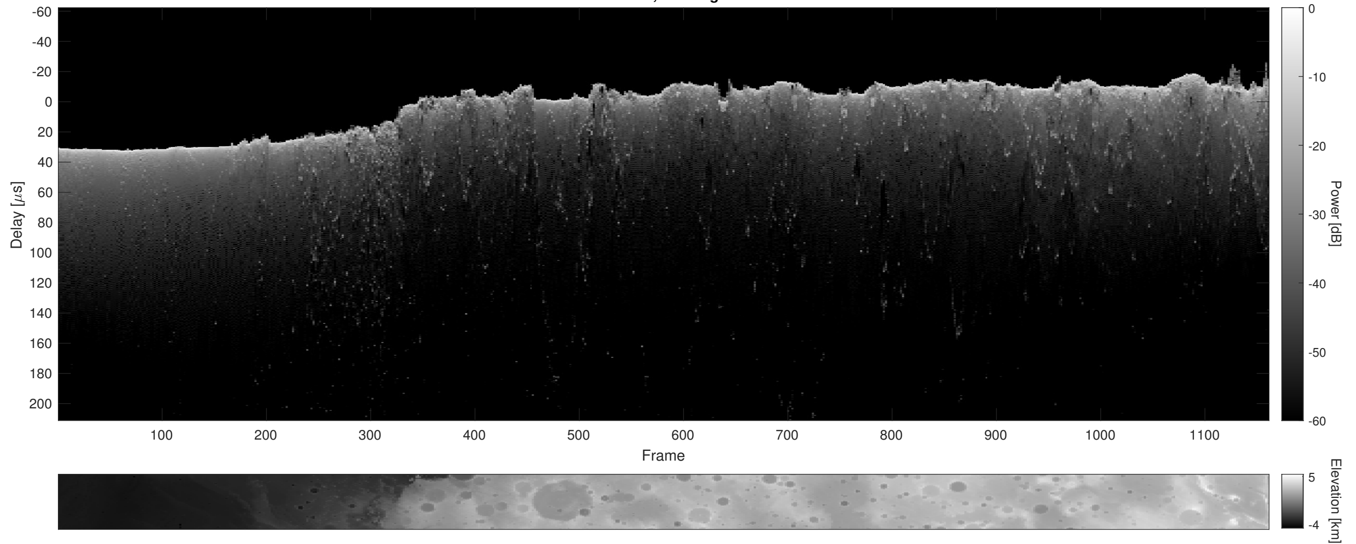
Orbit 7060, Cluttergram
