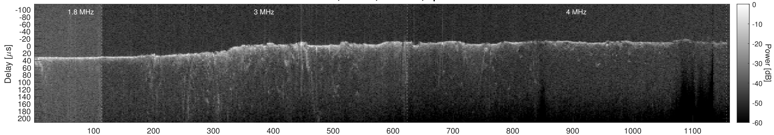
Orbit 7060, Cluttergram
