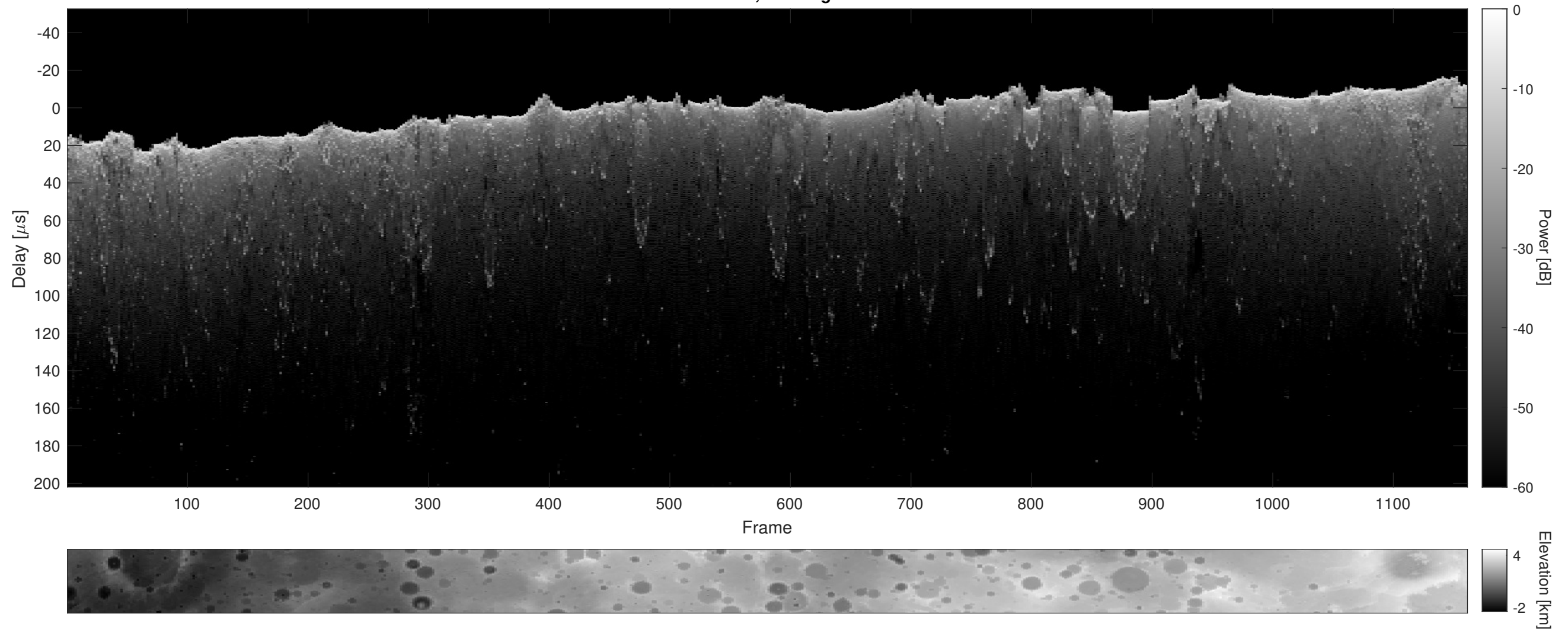
Orbit 7061, Cluttergram
