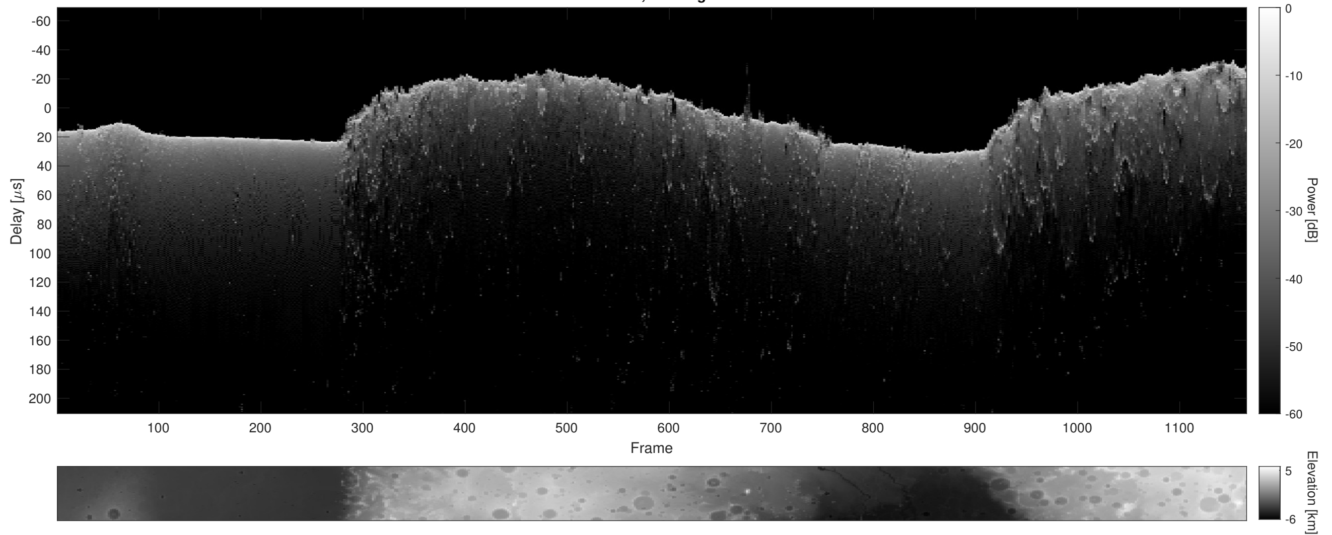
Orbit 7064, Cluttergram
