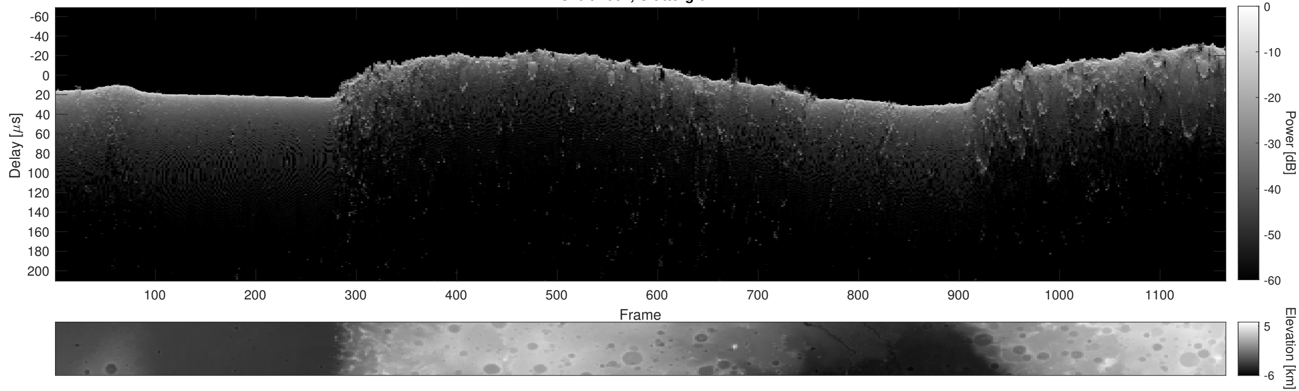
Orbit 7064, Cluttergram
