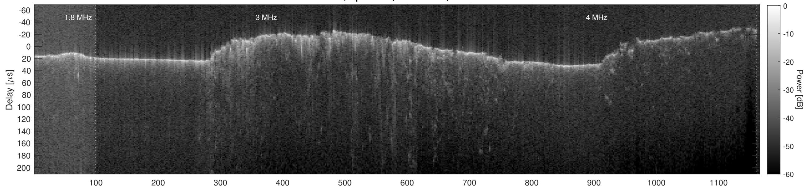
Orbit 7064, Cluttergram
