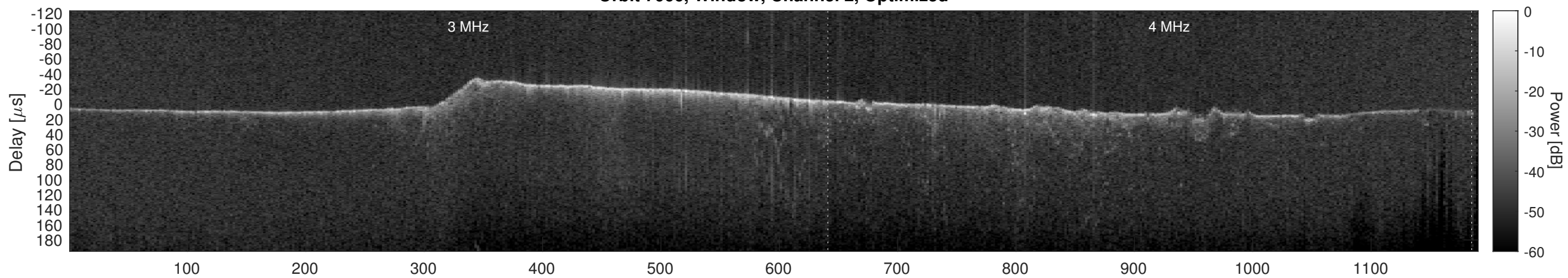
Orbit 7066, Cluttergram
