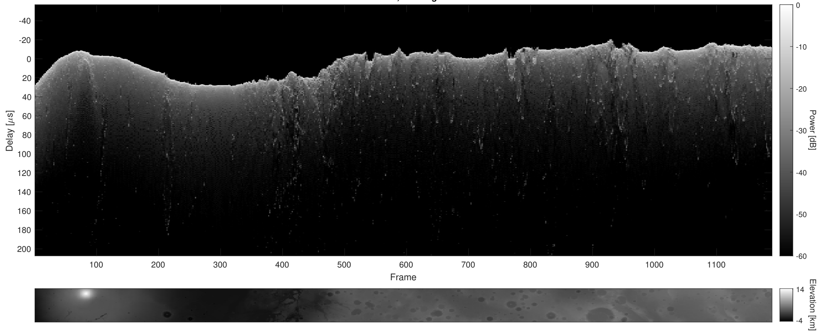
Orbit 7067, Cluttergram
