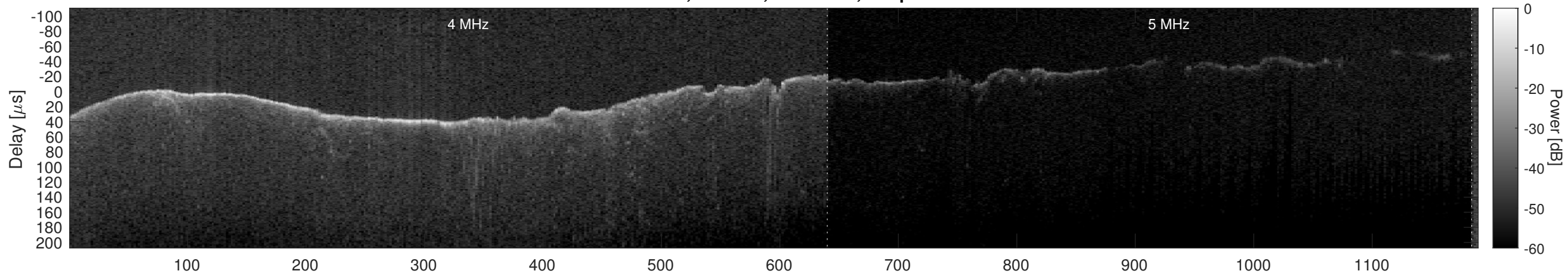
Orbit 7067, Window, Channel 1, Optimized
