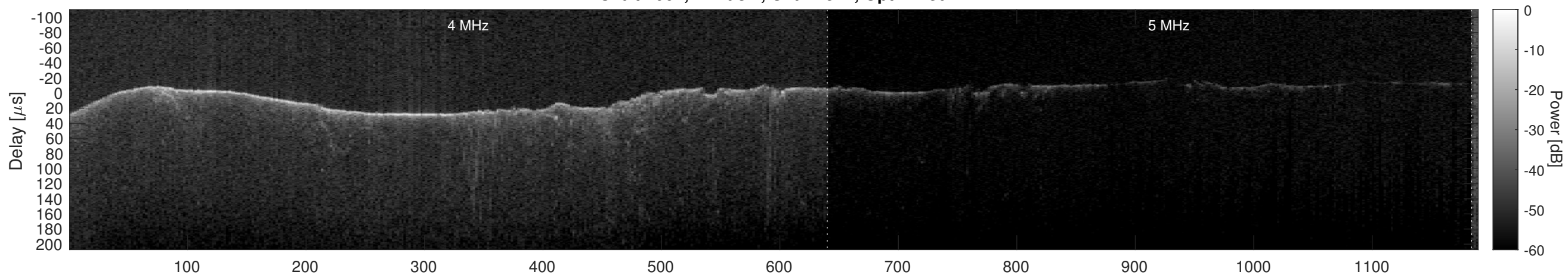
Orbit 7067, Cluttergram
