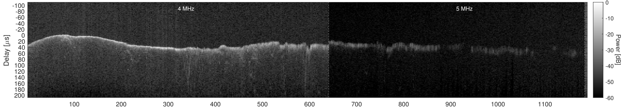
Orbit 7067, Window, Channel 1, Chapman
