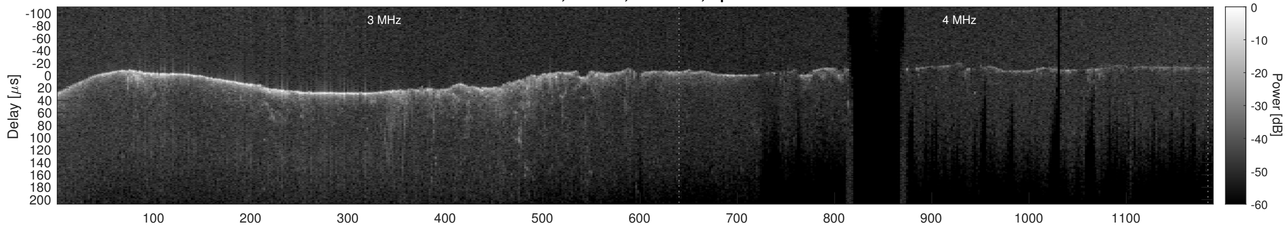
Orbit 7067, Cluttergram
