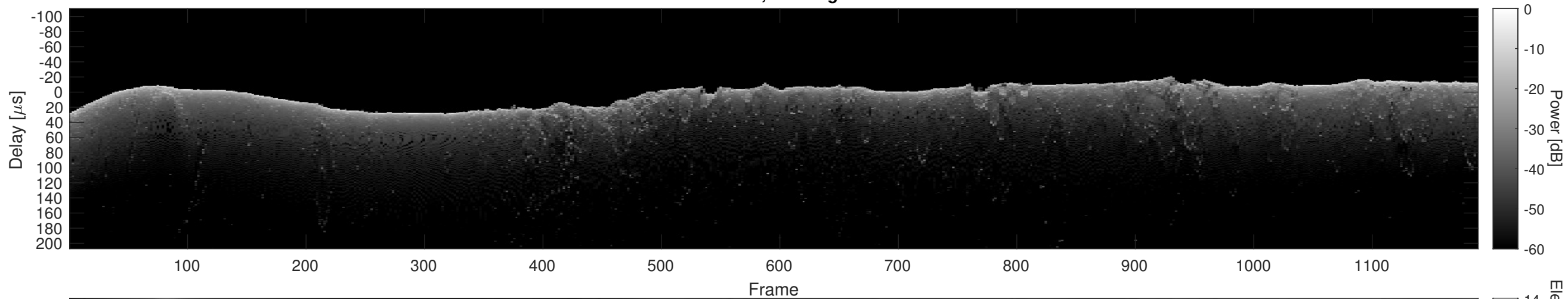
Orbit 7067, Cluttergram
