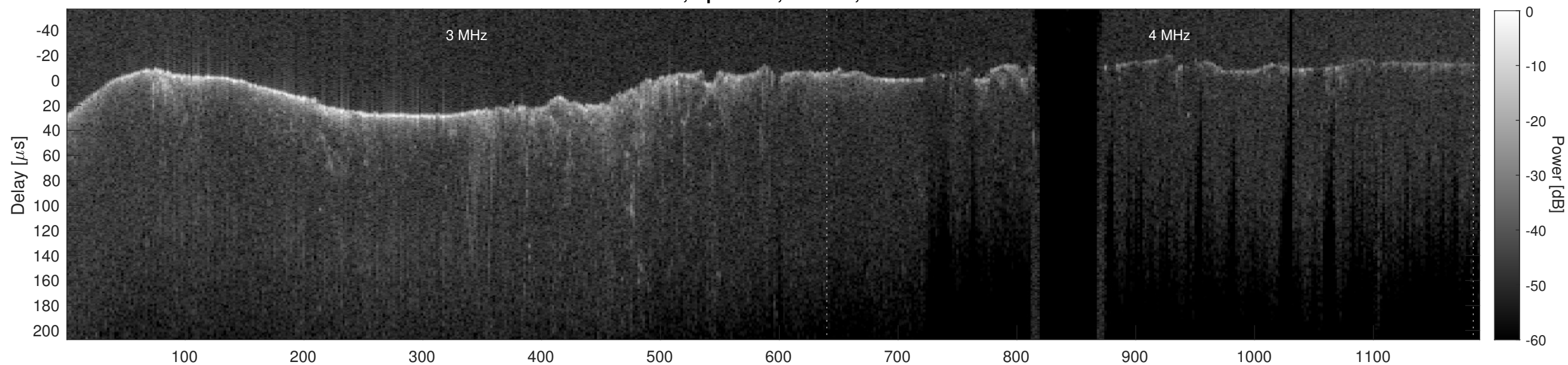
Orbit 7067, Cluttergram
