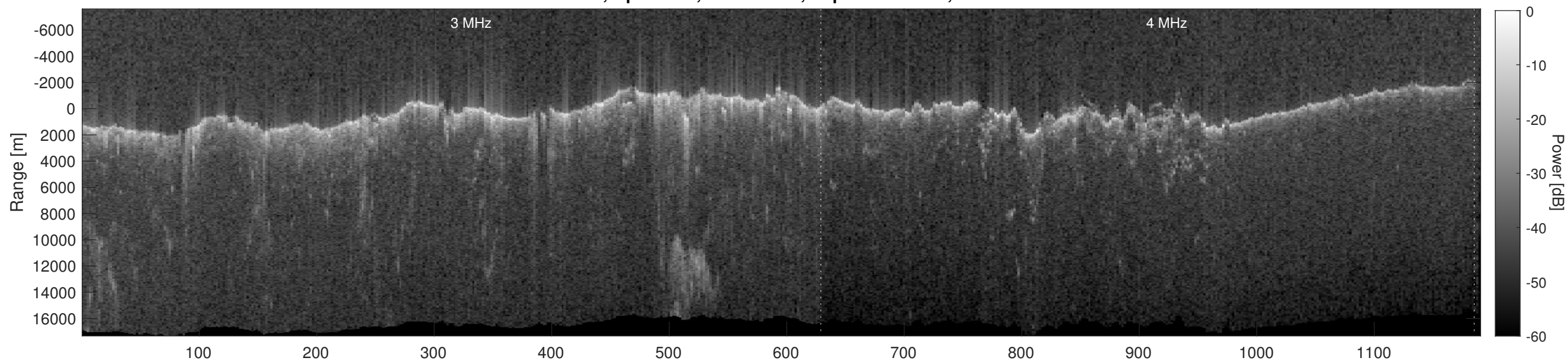
Orbit 7068, Depth-Corrected Cluttergram
