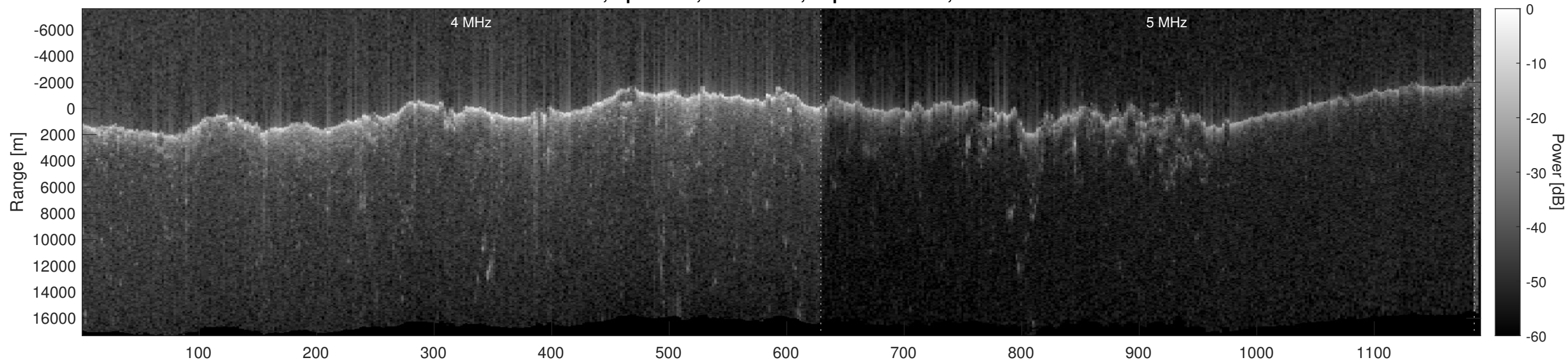
Orbit 7068, Optimized, No Window, Depth-Corrected, Channel 2
