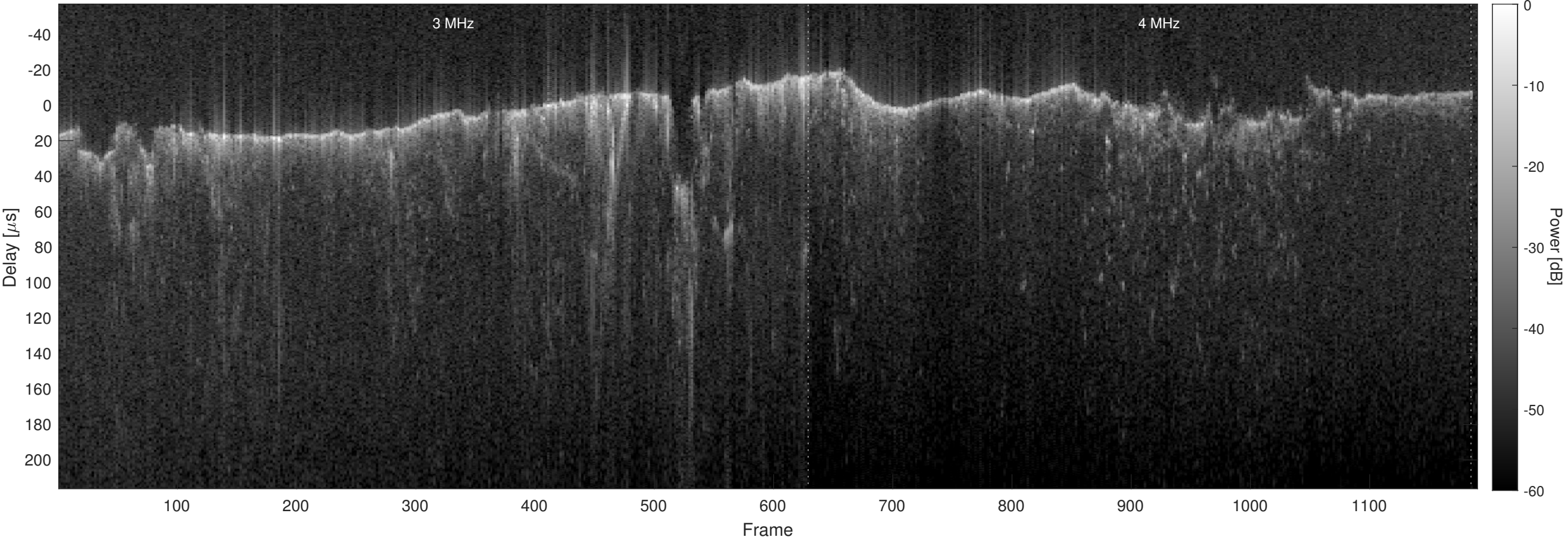
Orbit 7069, Optimized, No Window, Channel 2
