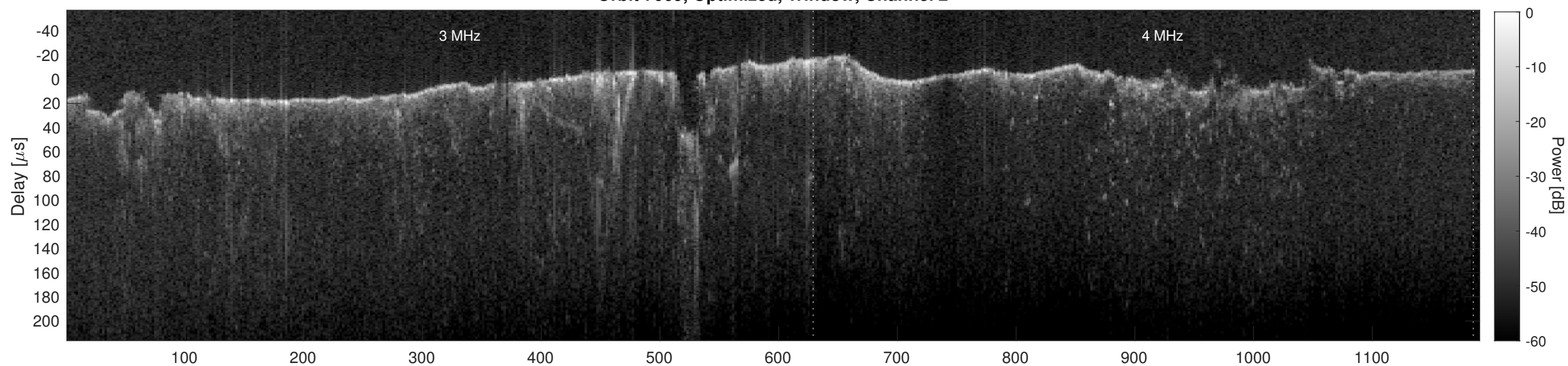
Orbit 7069, Cluttergram
