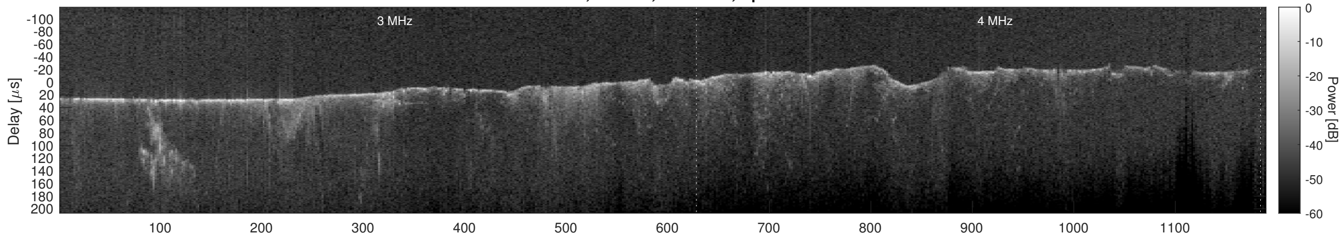
Orbit 7070, Cluttergram
