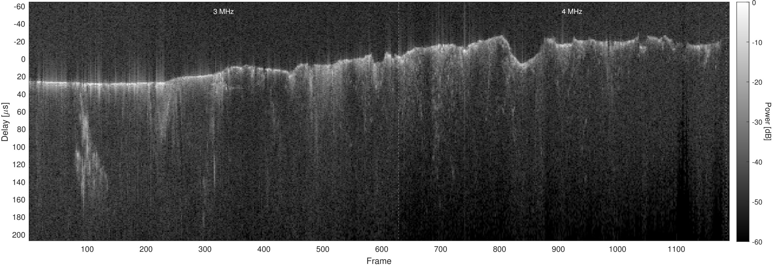
Orbit 7070, Optimized, No Window, Channel 2
