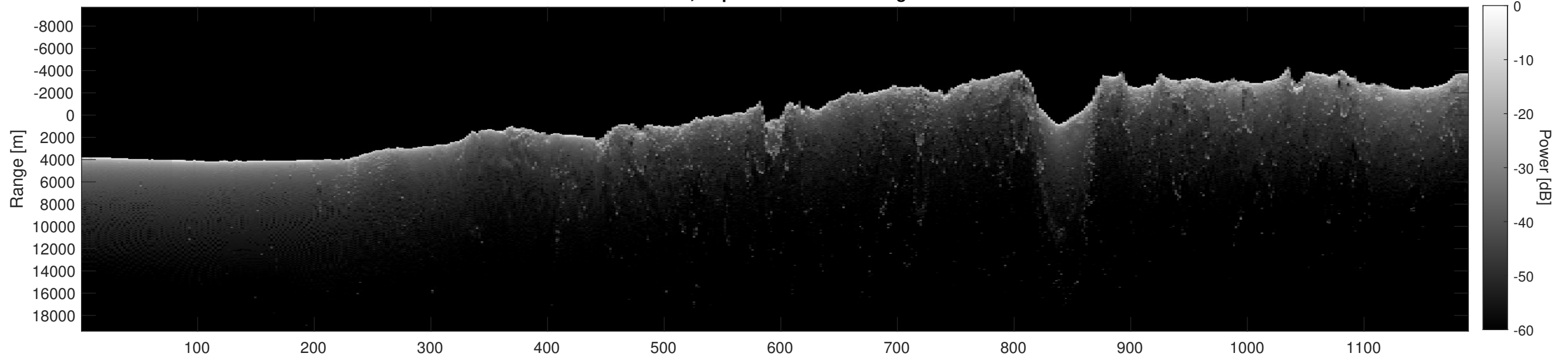
Orbit 7070, Depth-Corrected Cluttergram
