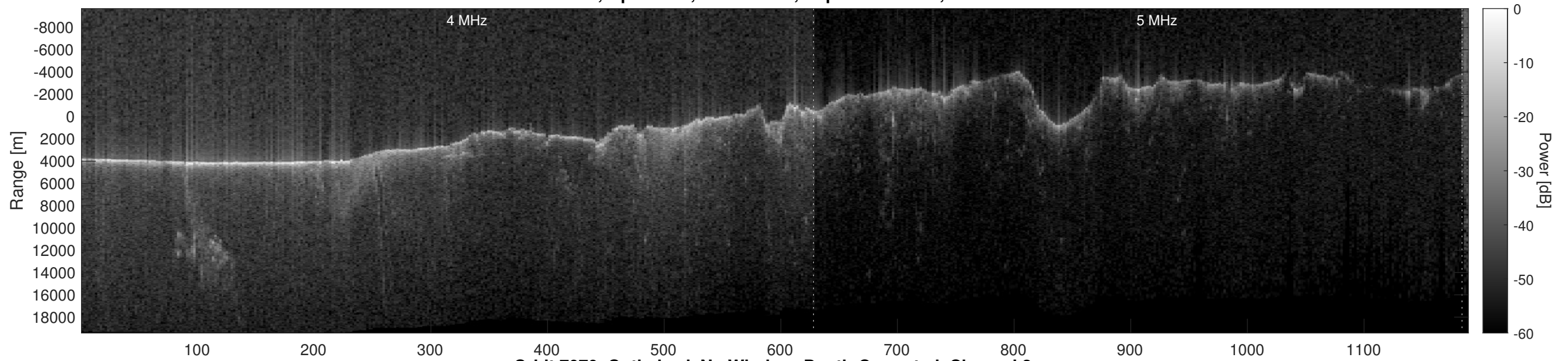
Orbit 7070, Optimized, No Window, Depth-Corrected, Channel 2
