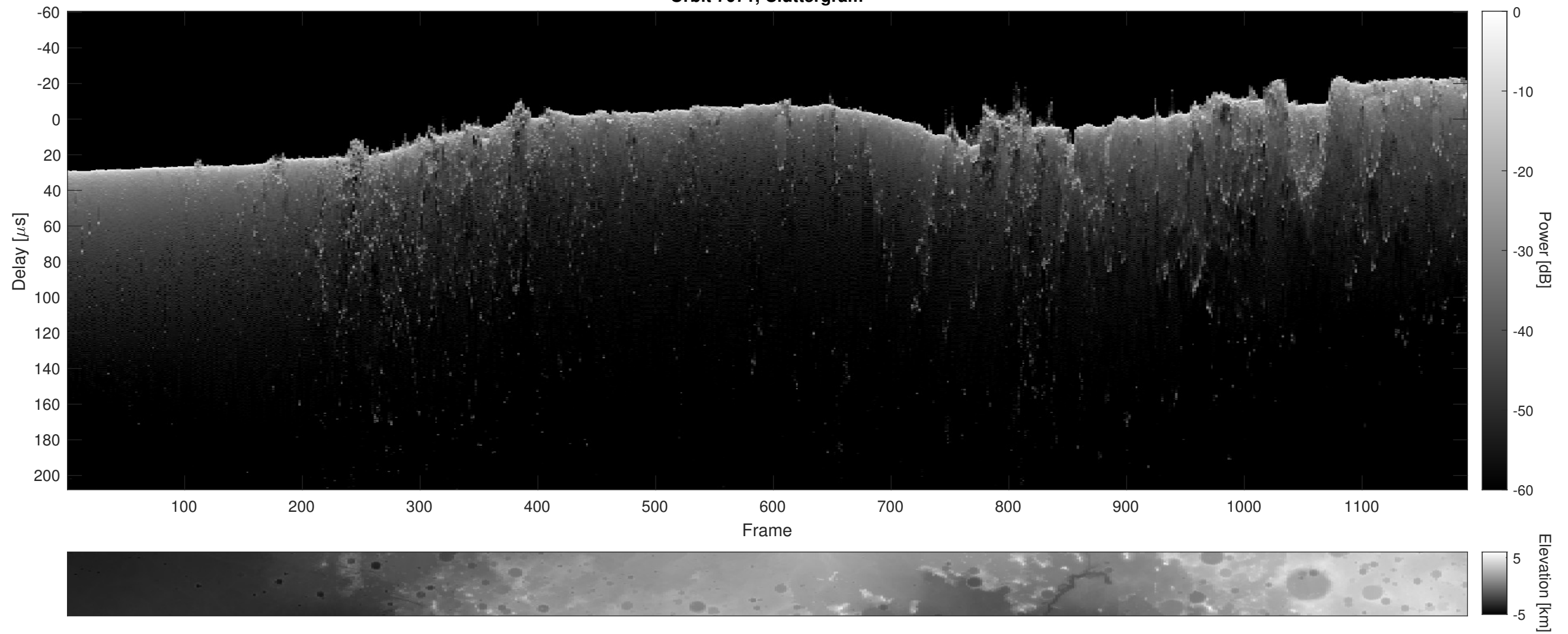
Orbit 7071, Cluttergram
