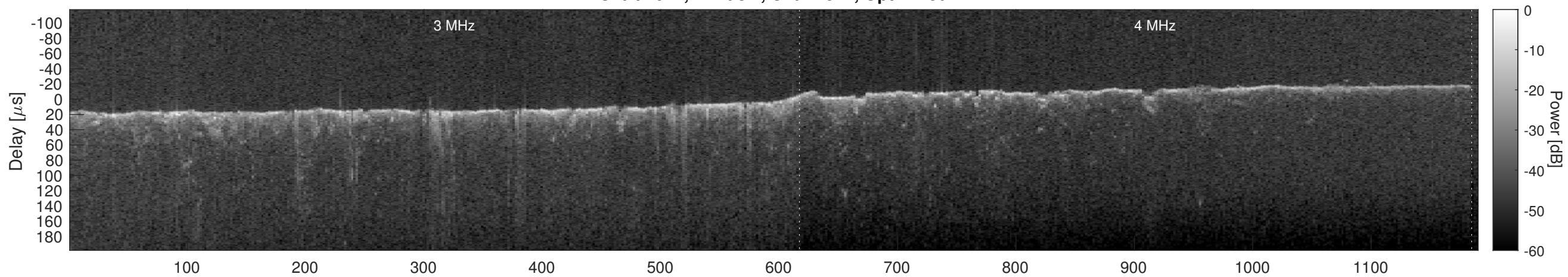
Orbit 7072, Cluttergram
