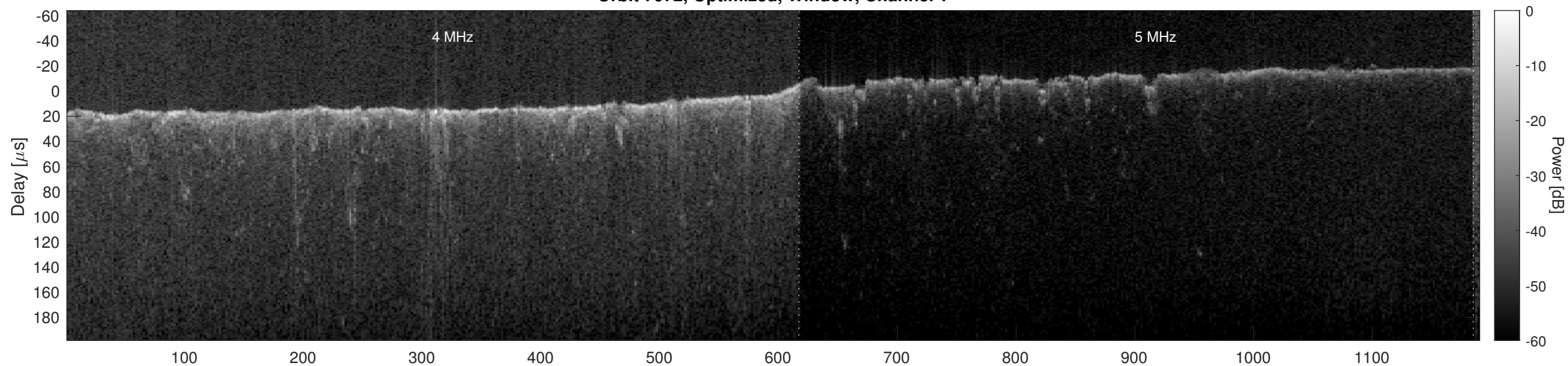
Orbit 7072, Optimized, Window, Channel 2
