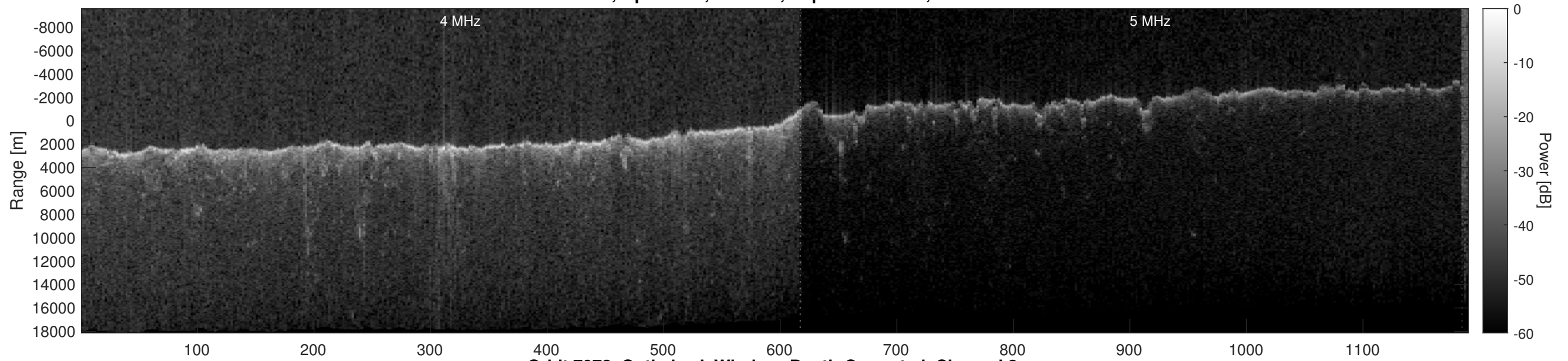
Orbit 7072, Optimized, Window, Depth-Corrected, Channel 2
