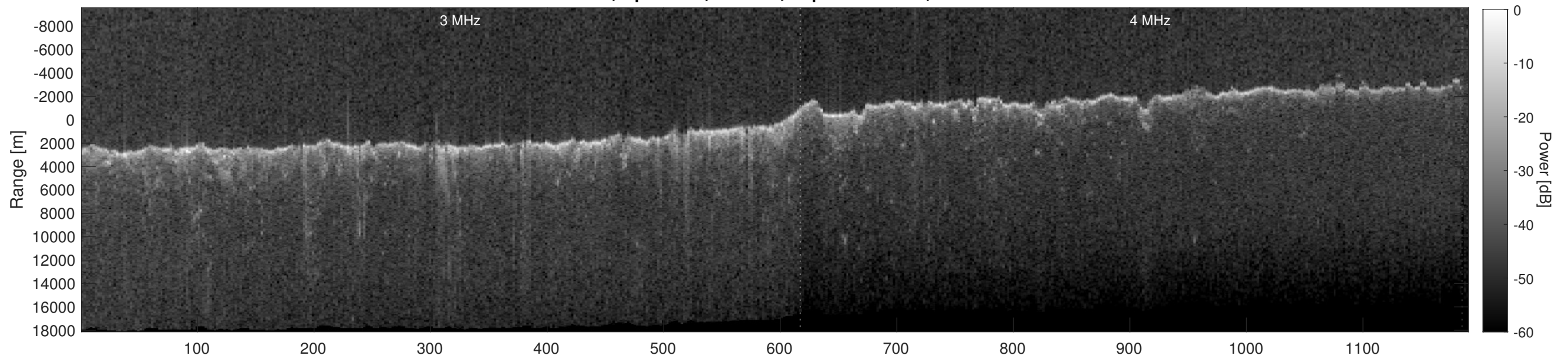
Orbit 7072, Depth-Corrected Cluttergram
