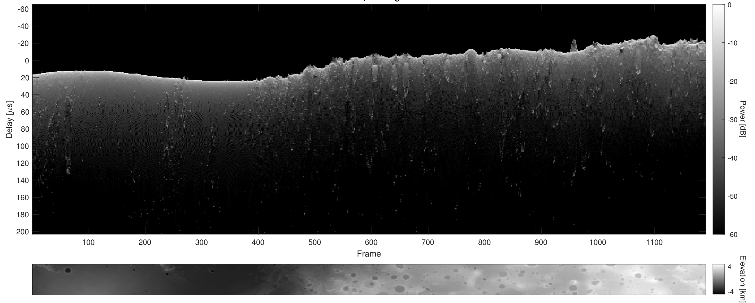
Orbit 7074, Cluttergram
