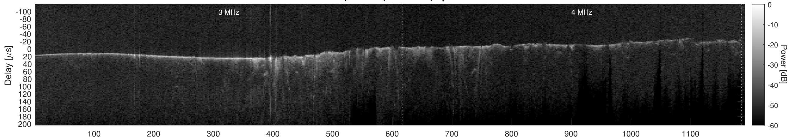
Orbit 7074, Cluttergram
