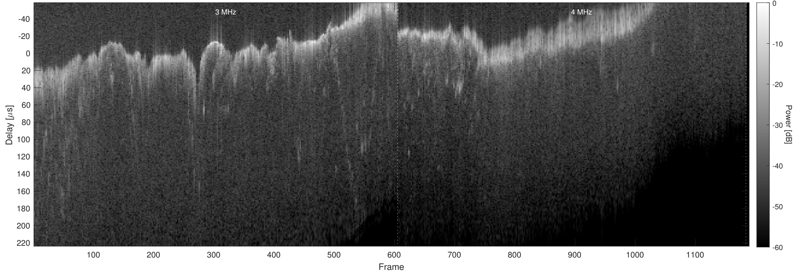
Orbit 7075, Chapman, No Window, Channel 2
