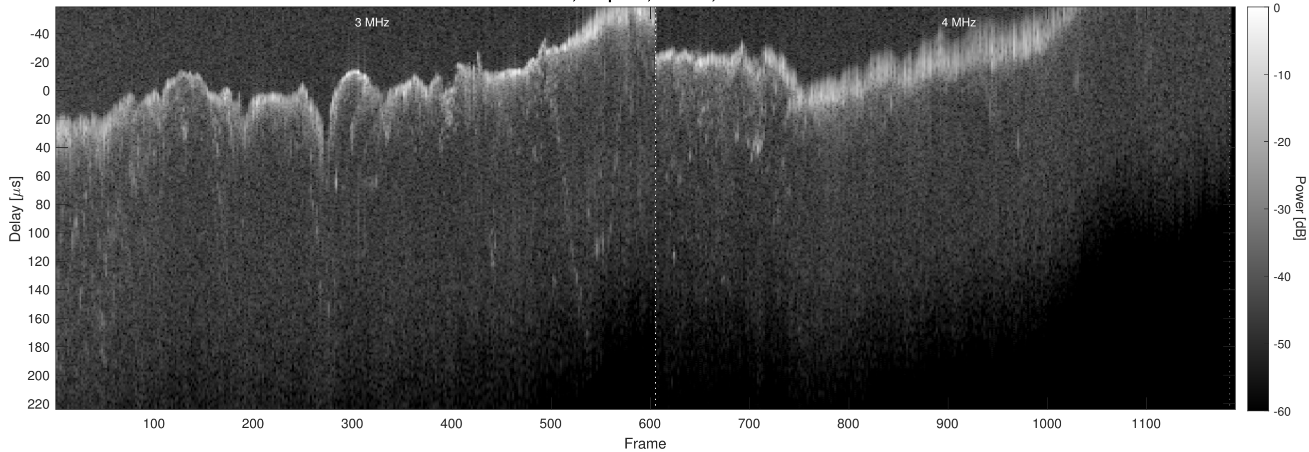
Orbit 7075, Chapman, Window, Channel 2
