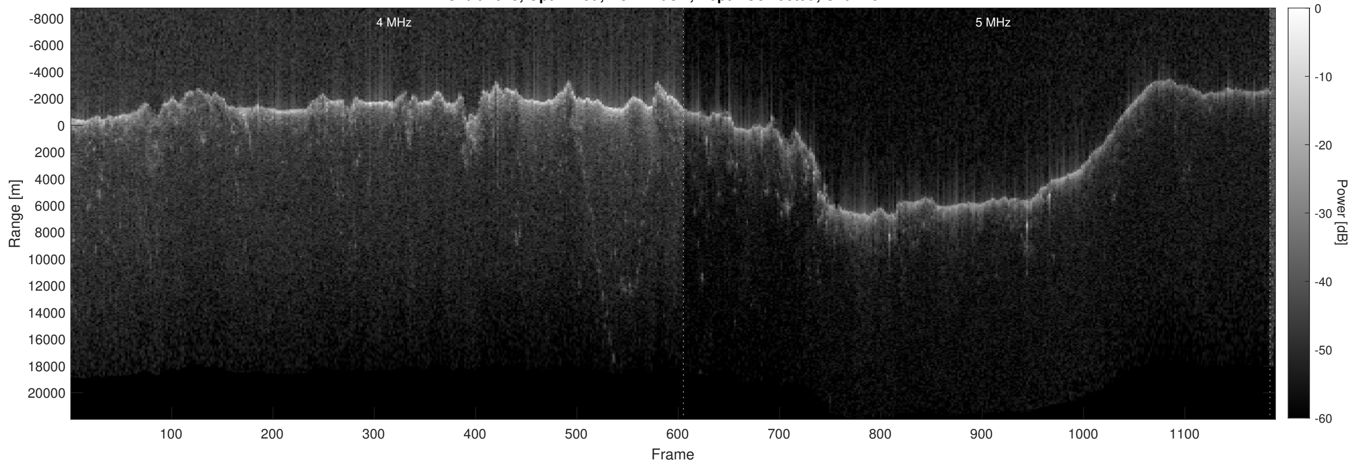
Orbit 7075, Optimized, No Window, Depth-Corrected, Channel 2
