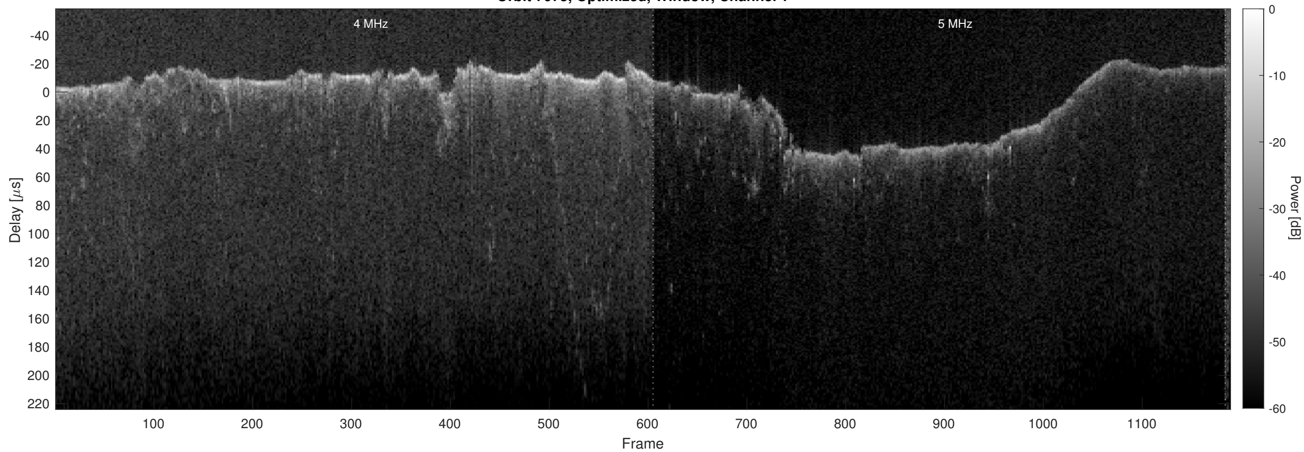
Orbit 7075, Optimized, Window, Channel 2
