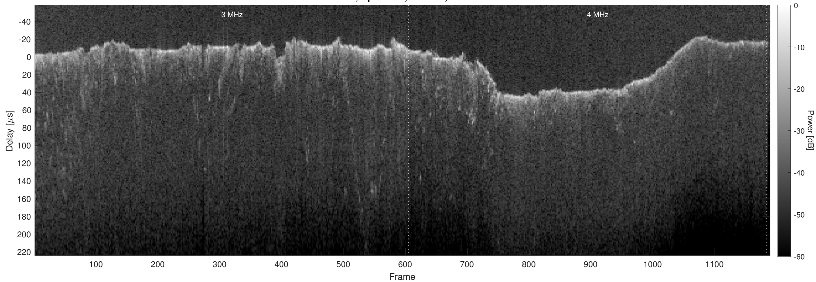
Orbit 7075, Optimized, Window, Channel 2
