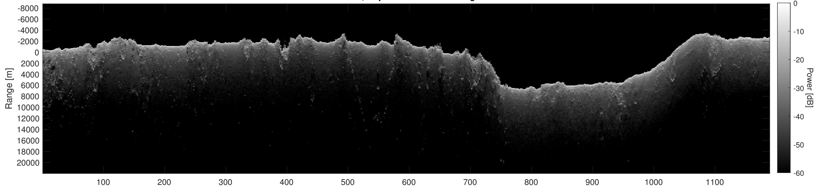
Orbit 7075, Depth-Corrected Cluttergram
