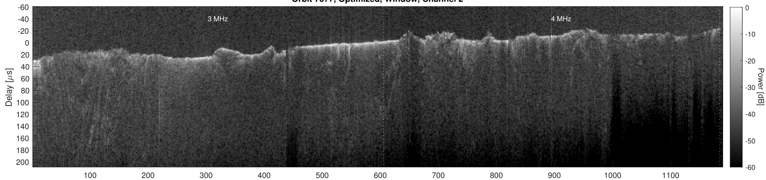
Orbit 7077, Cluttergram
