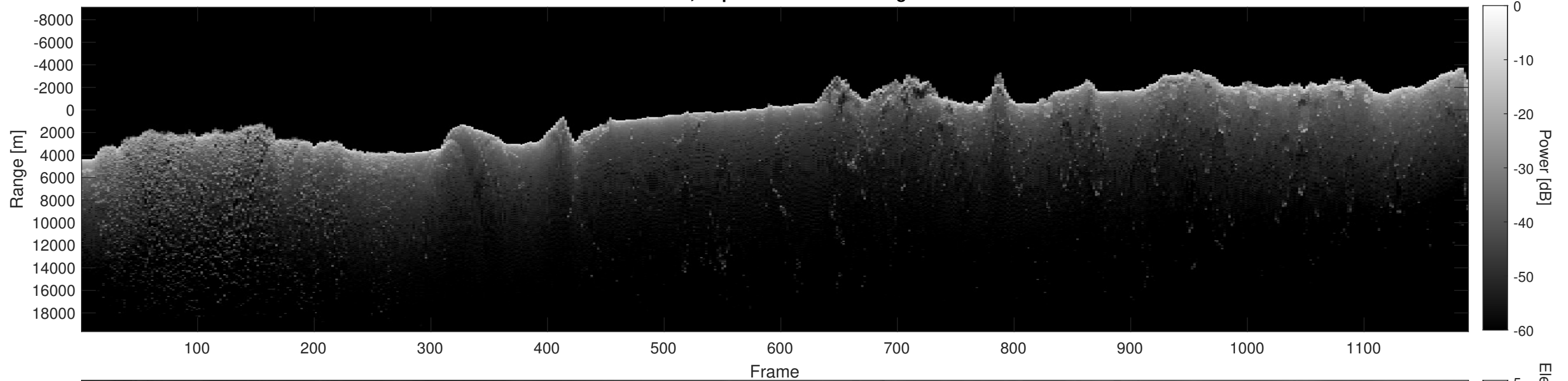
Orbit 7077, Depth-Corrected Cluttergram
