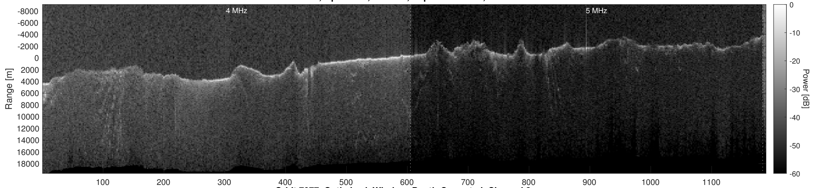
Orbit 7077, Optimized, Window, Depth-Corrected, Channel 2
