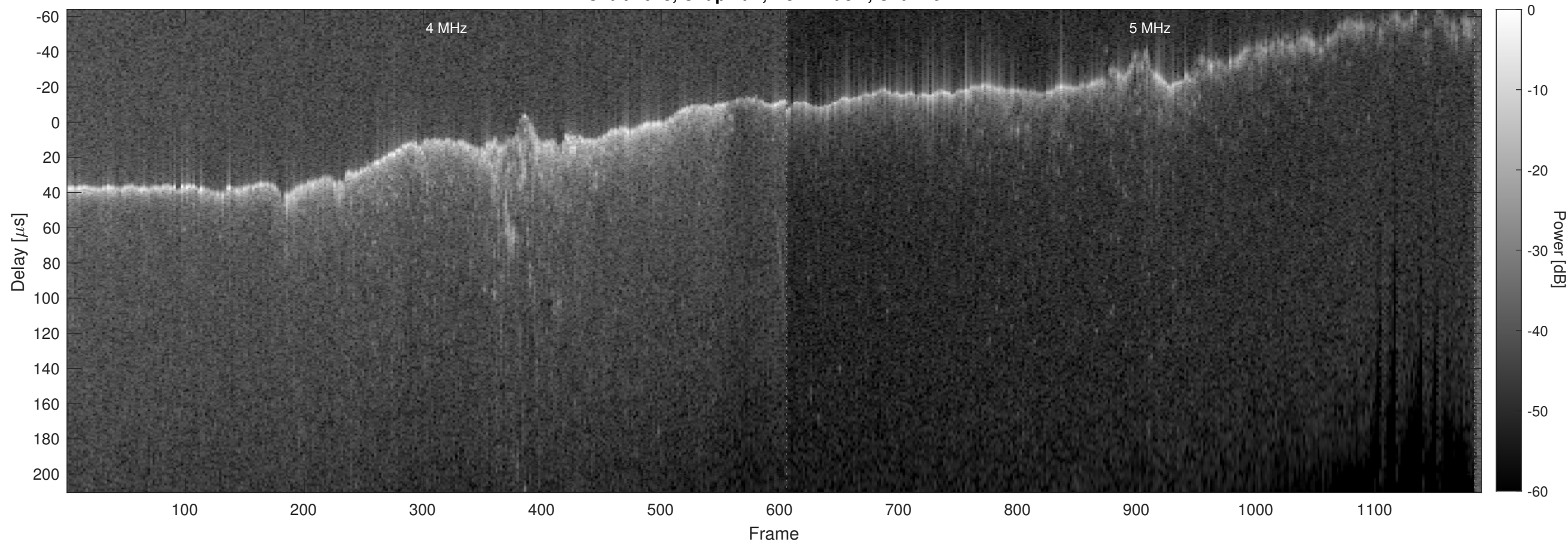
Orbit 7078, Chapman, No Window, Channel 2
