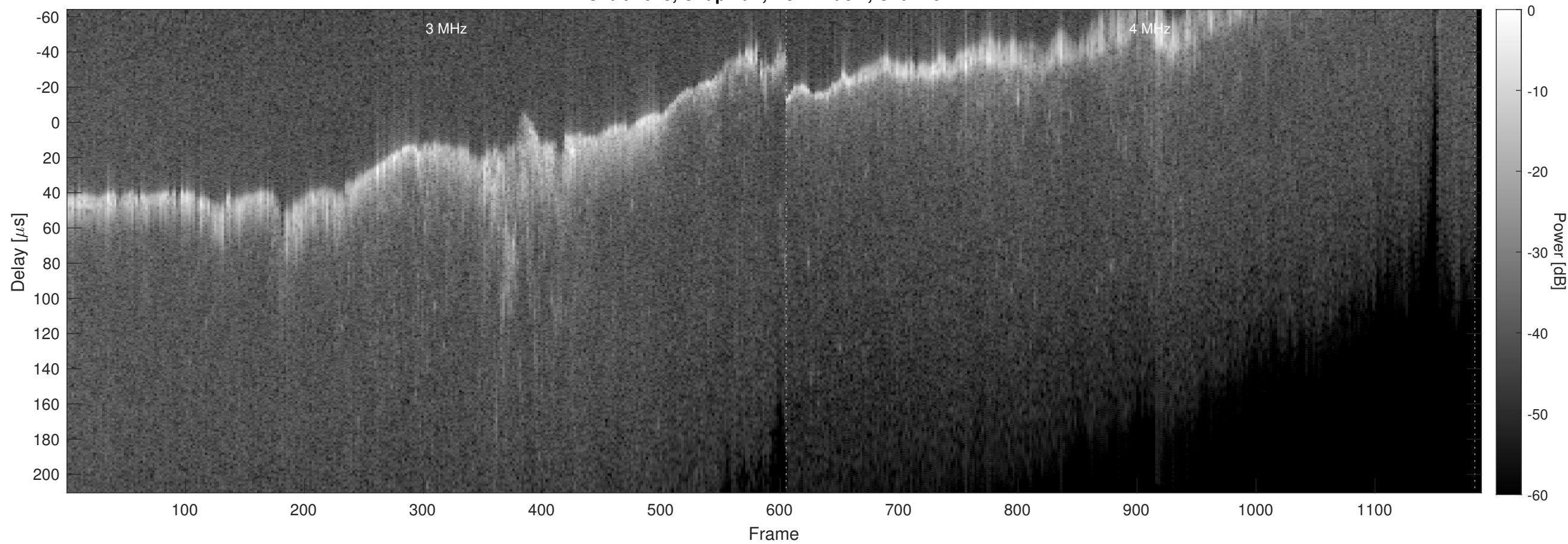
Orbit 7078, Chapman, No Window, Channel 2
