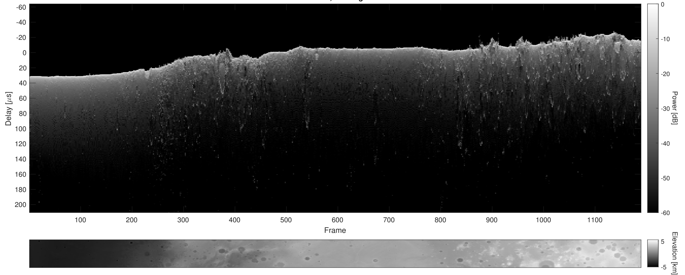
Orbit 7078, Cluttergram
