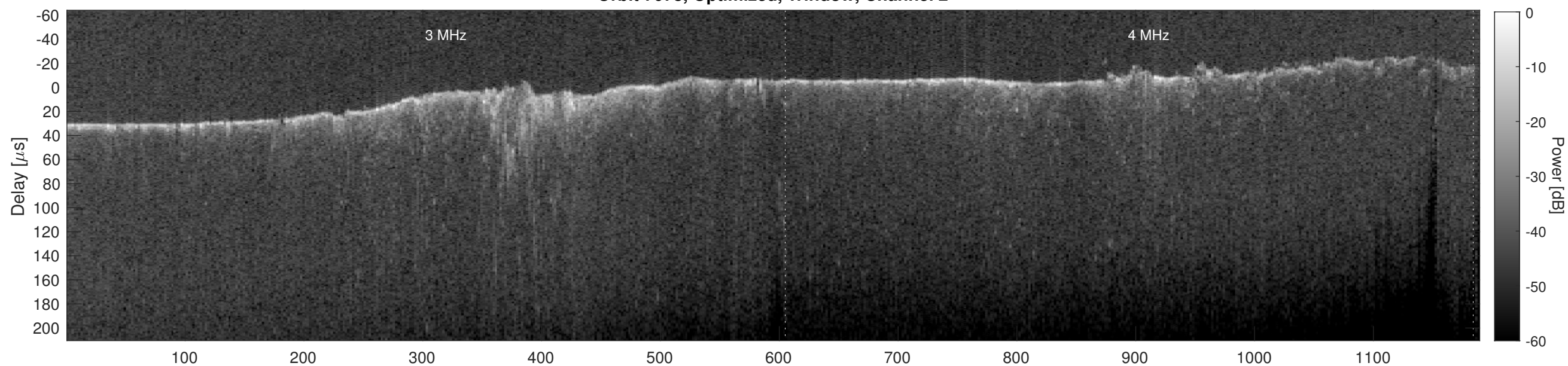
Orbit 7078, Cluttergram
