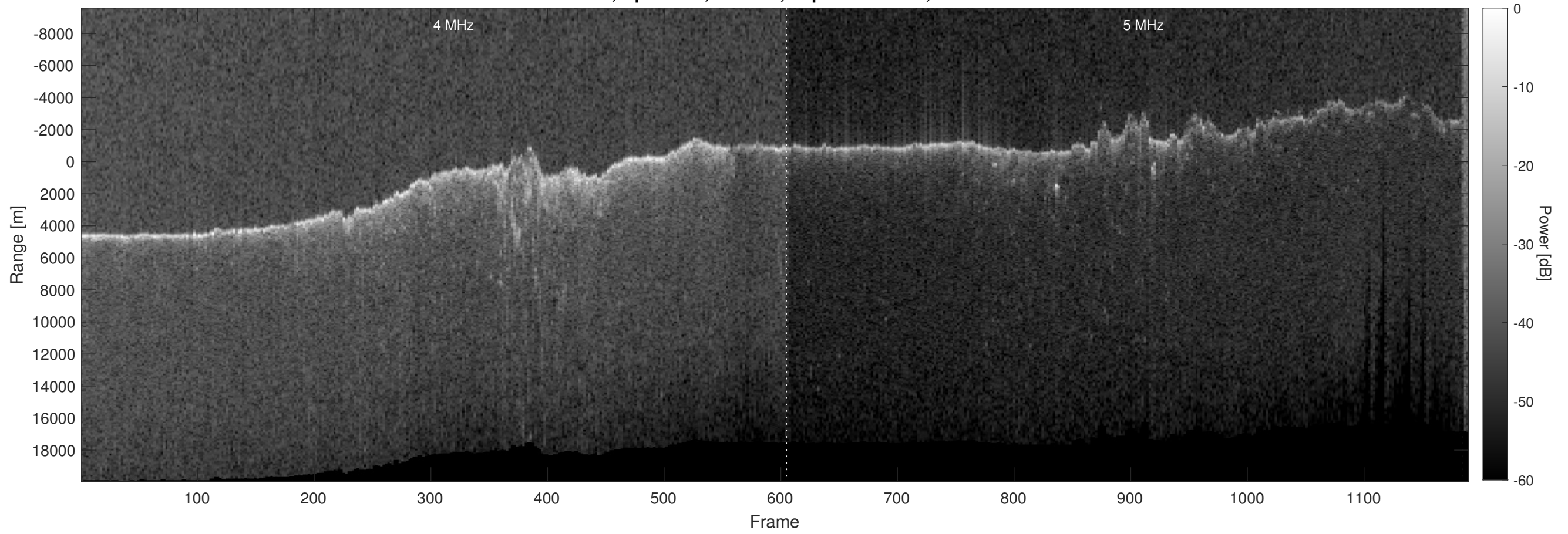
Orbit 7078, Optimized, Window, Depth-Corrected, Channel 2
