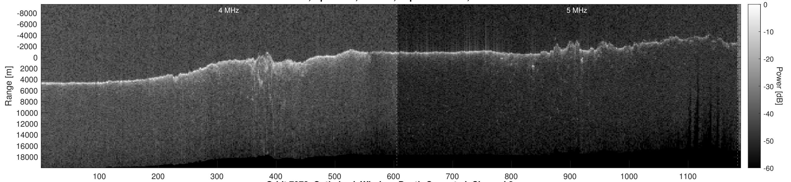
Orbit 7078, Optimized, Window, Depth-Corrected, Channel 2
