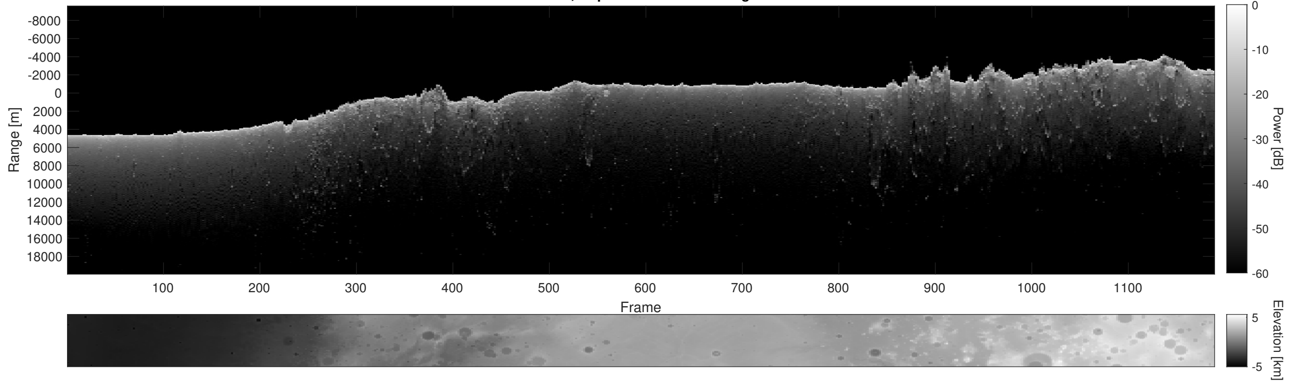
Orbit 7078, Depth-Corrected Cluttergram
