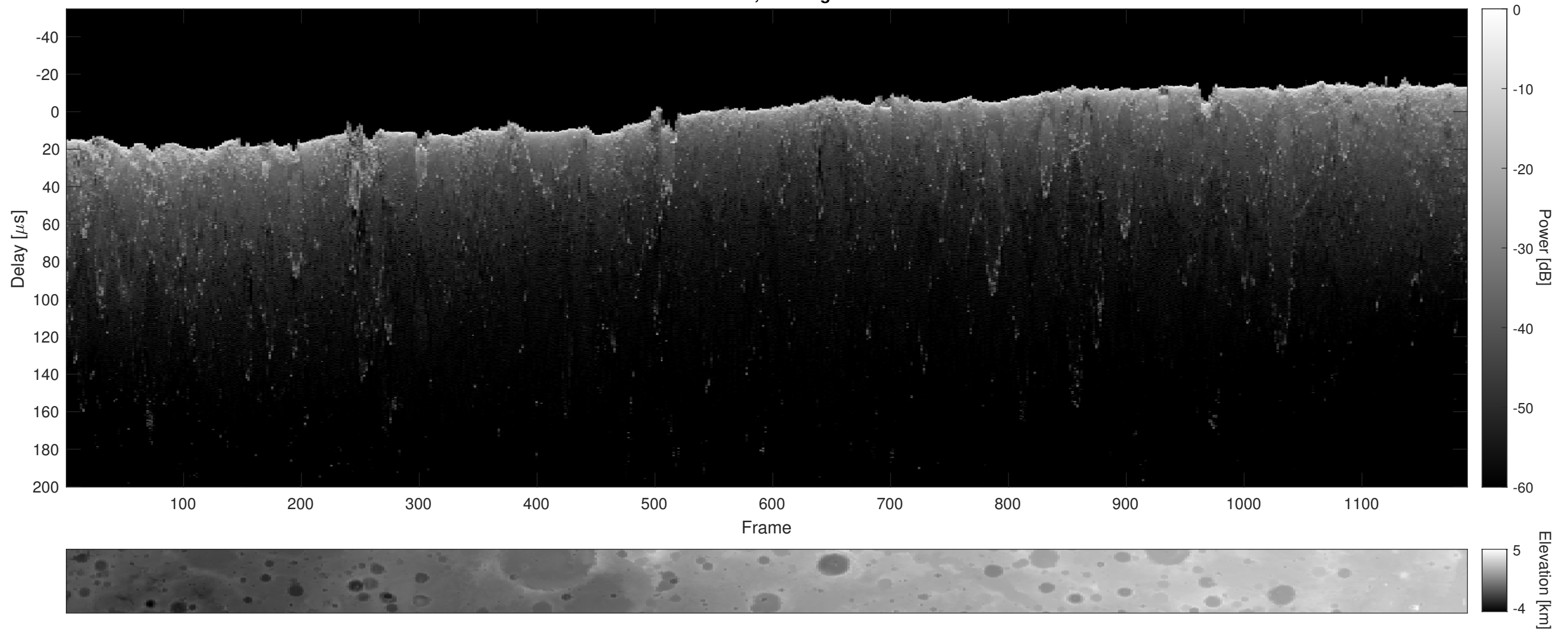
Orbit 7079, Cluttergram
