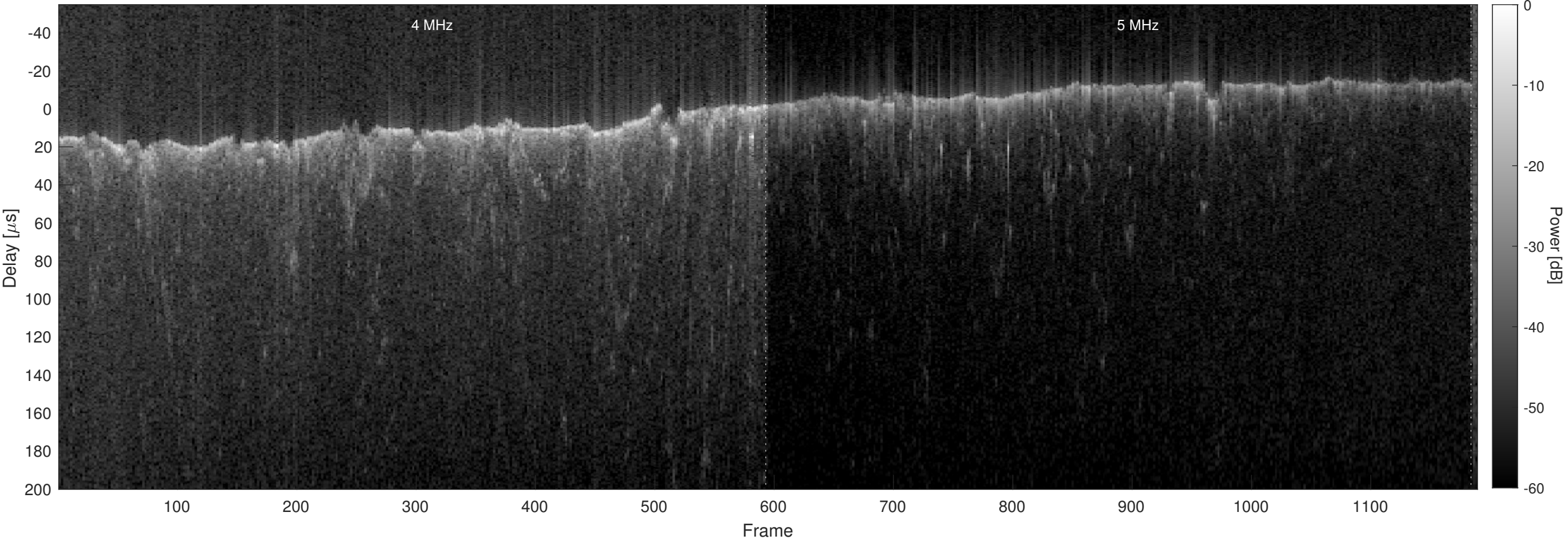
Orbit 7079, Optimized, No Window, Channel 2
