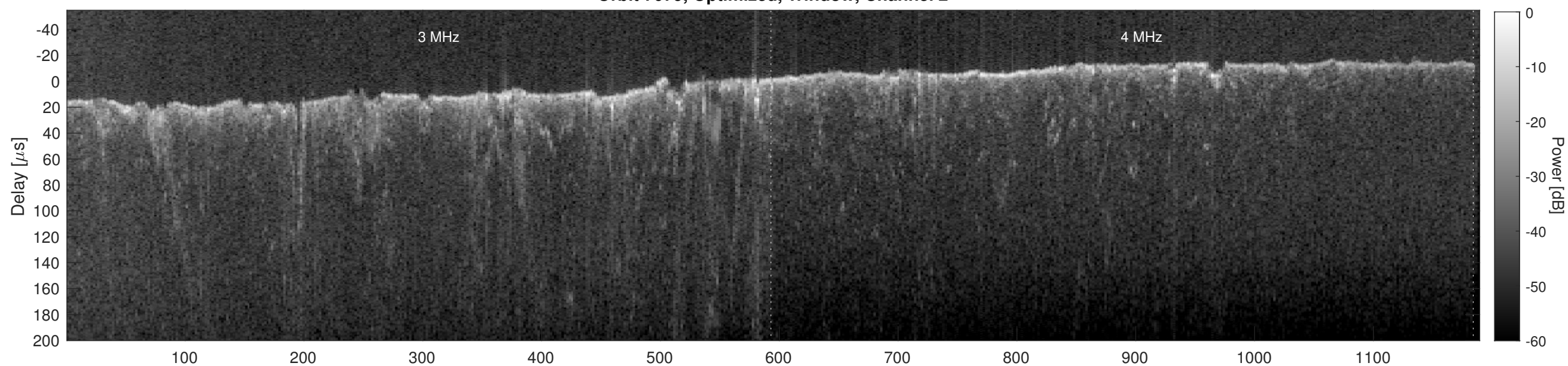
Orbit 7079, Cluttergram
