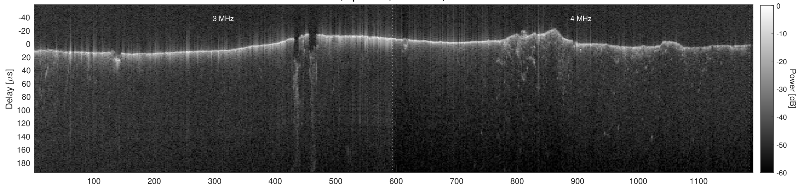
Orbit 7080, Cluttergram
