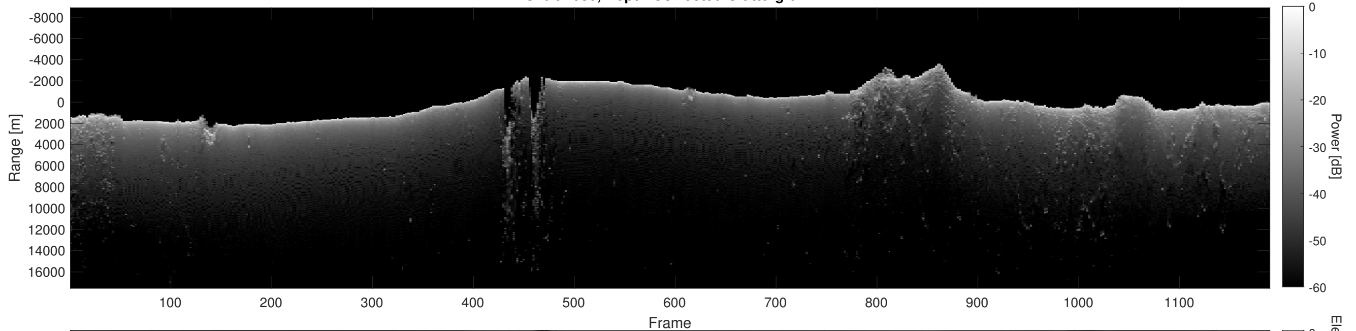
Orbit 7080, Depth-Corrected Cluttergram
