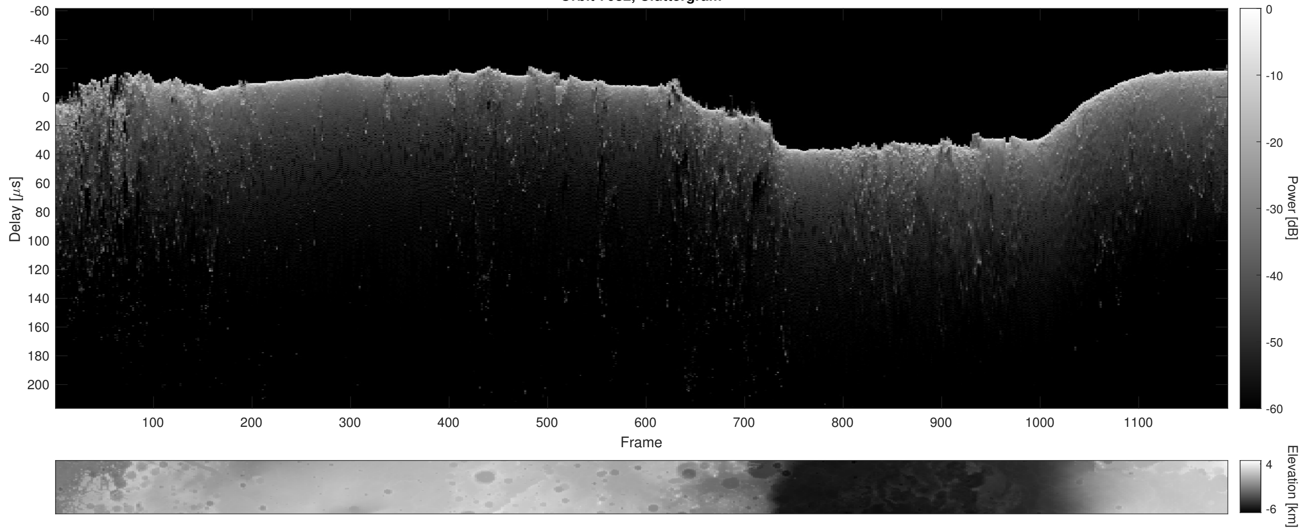
Orbit 7082, Cluttergram
