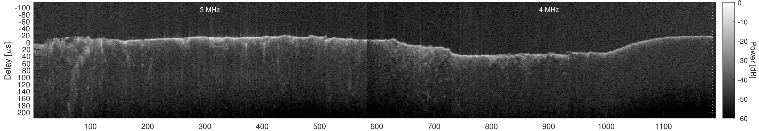
Orbit 7082, Cluttergram
