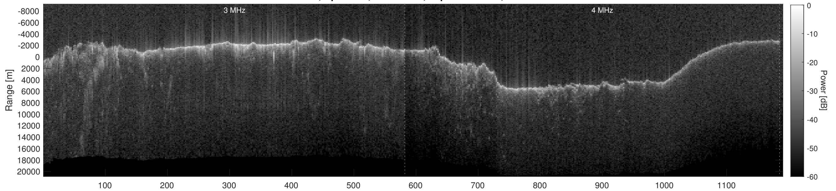
Orbit 7082, Depth-Corrected Cluttergram
