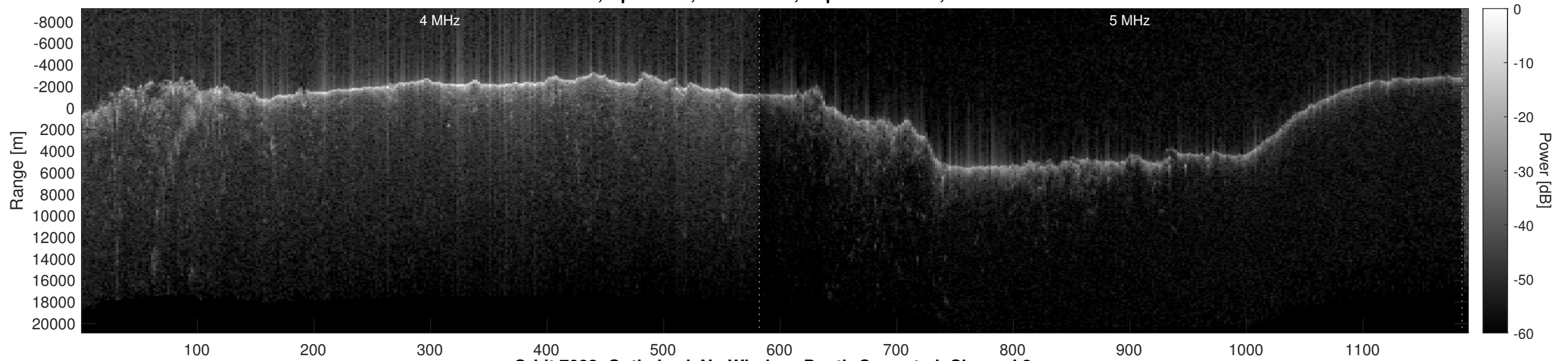
Orbit 7082, Optimized, No Window, Depth-Corrected, Channel 2
