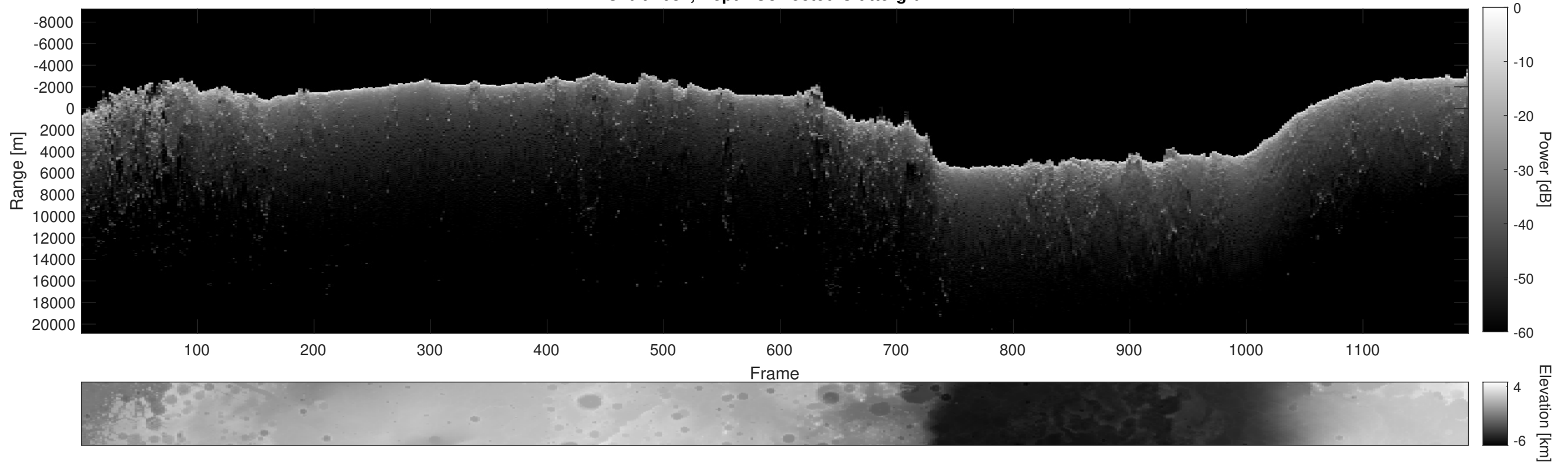
Orbit 7082, Depth-Corrected Cluttergram
