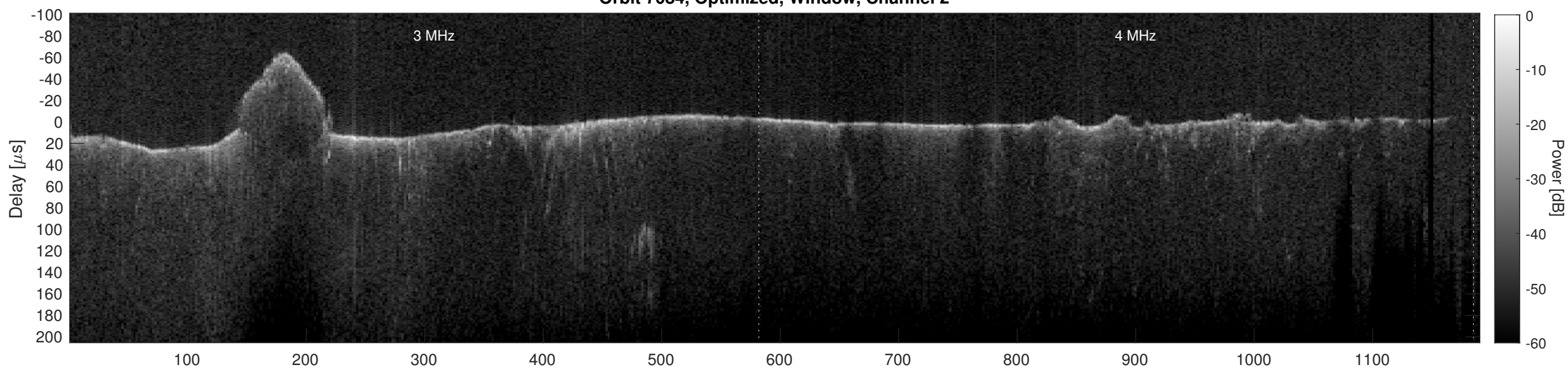
Orbit 7084, Cluttergram
