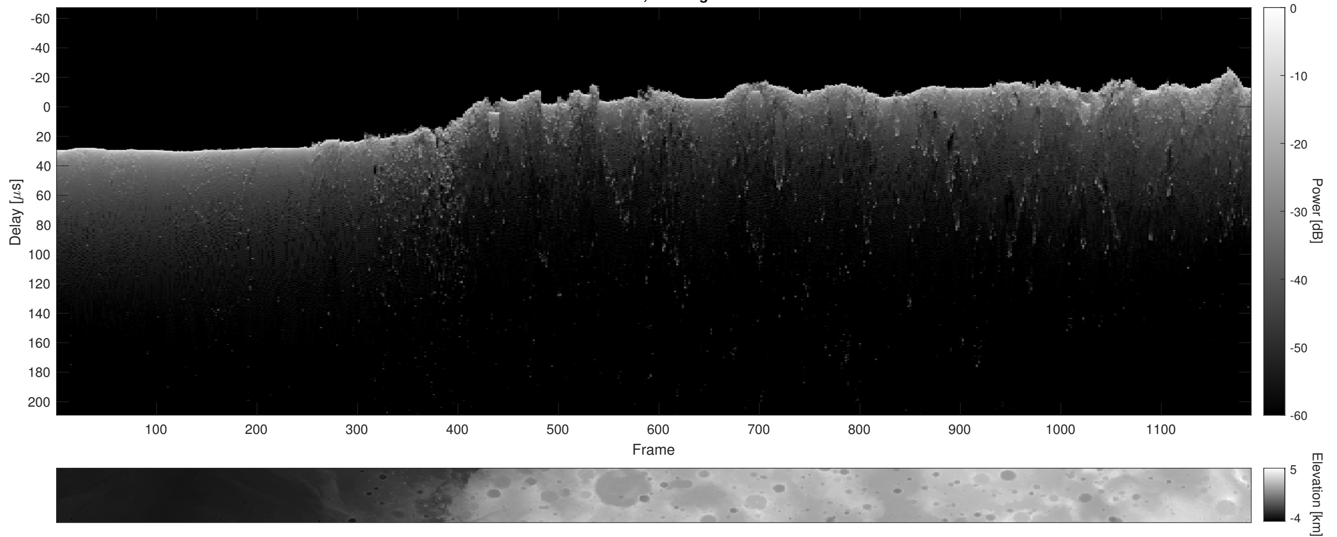
Orbit 7085, Cluttergram
