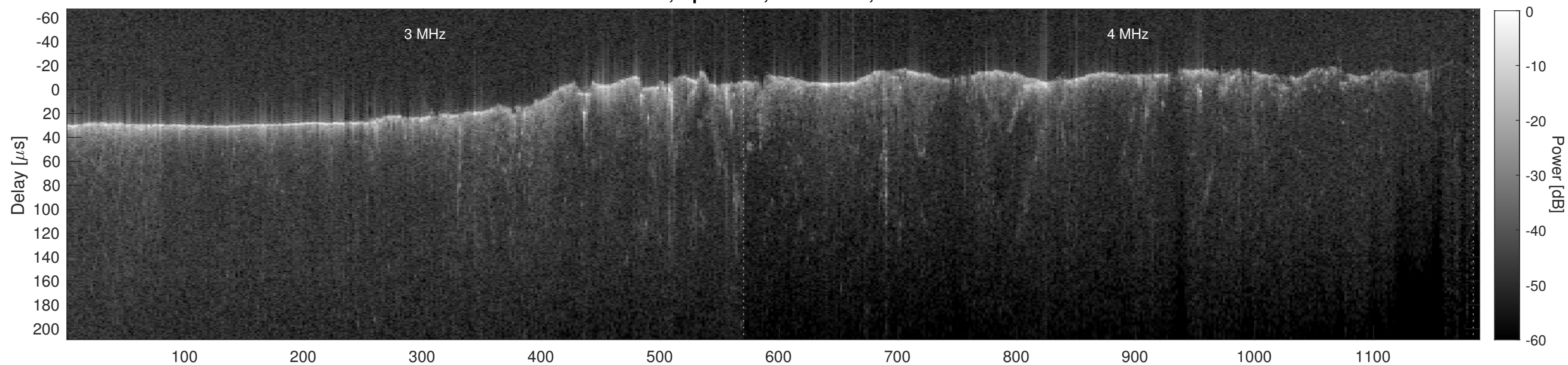
Orbit 7085, Cluttergram
