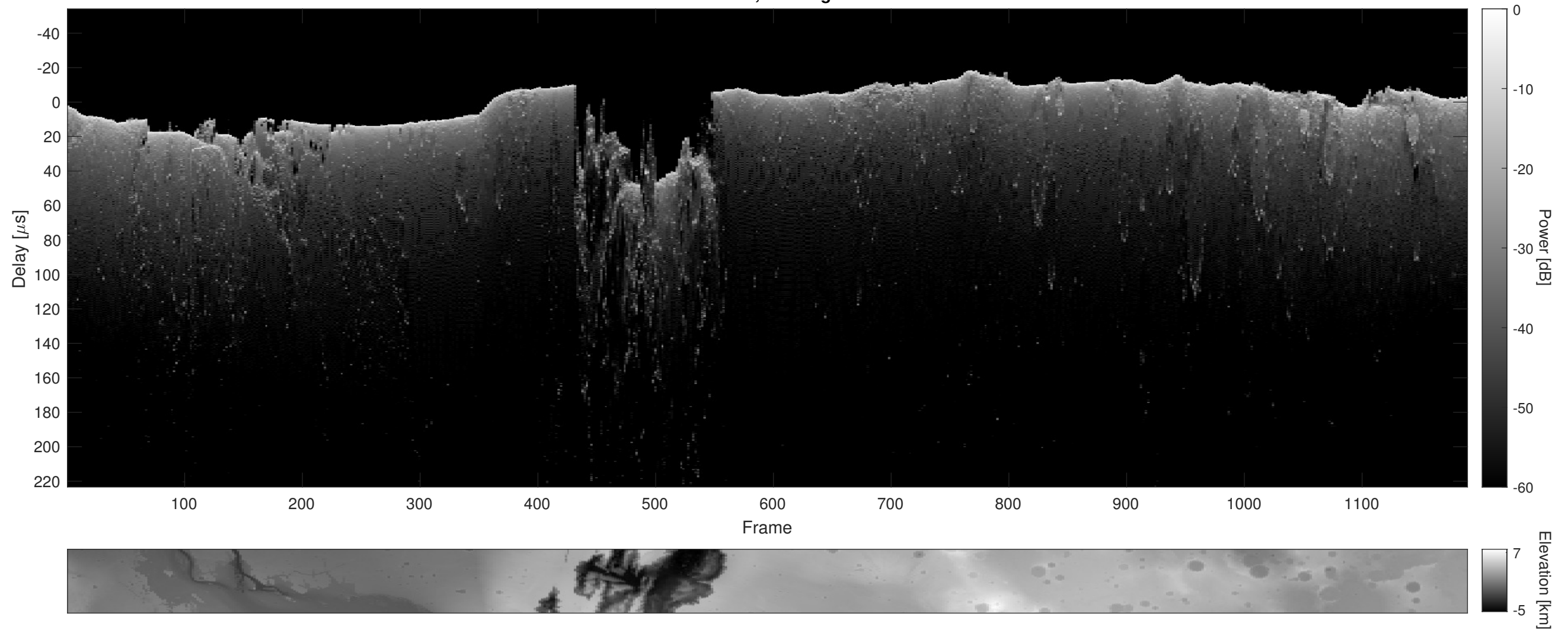
Orbit 7087, Cluttergram
