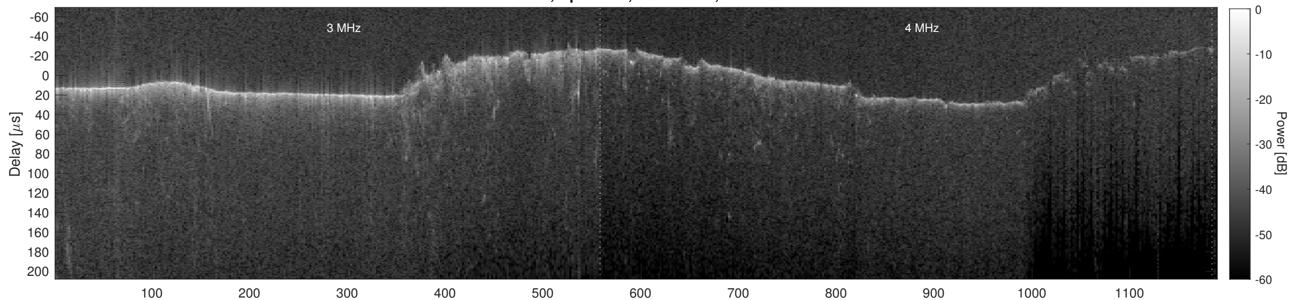
Orbit 7089, Cluttergram
