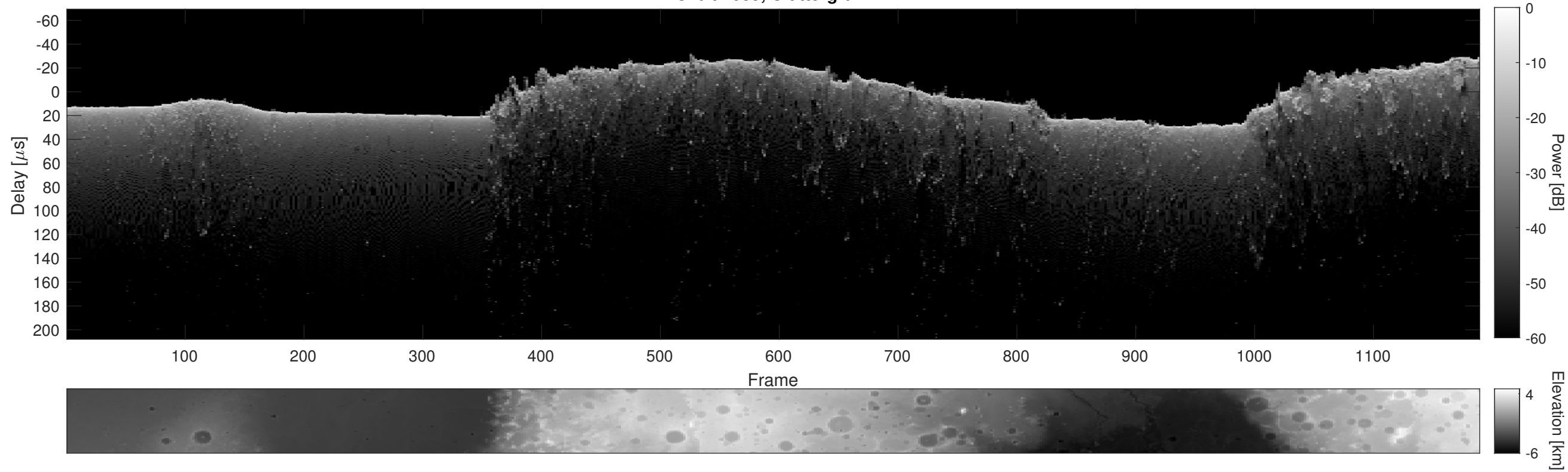
Orbit 7089, Cluttergram
