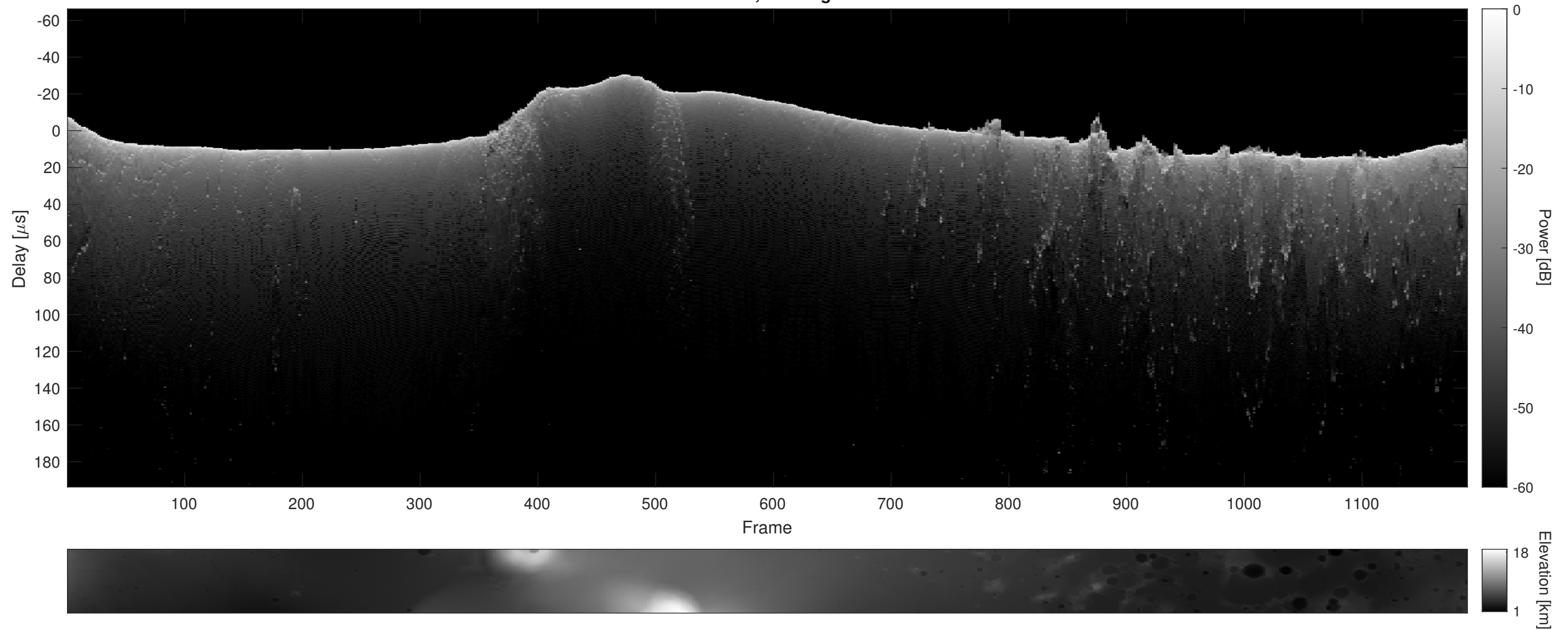
Orbit 7091, Cluttergram
