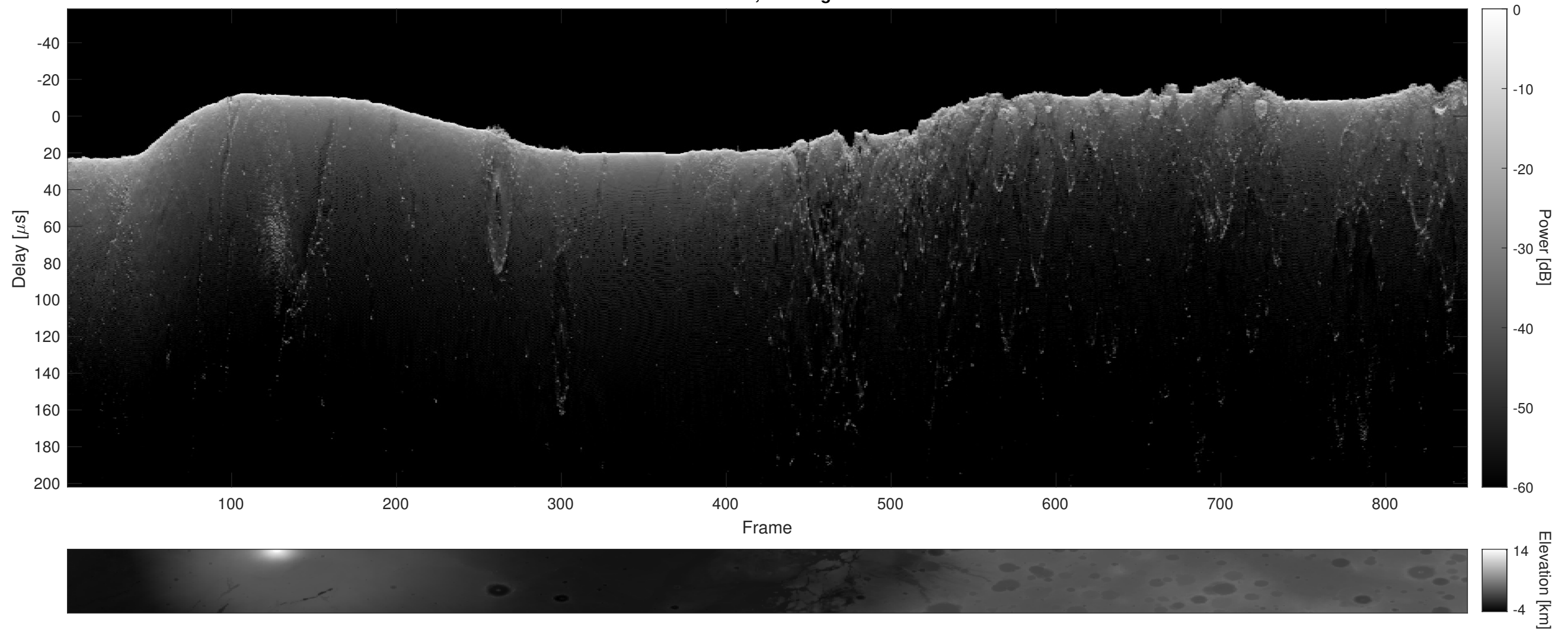
Orbit 7092, Cluttergram
