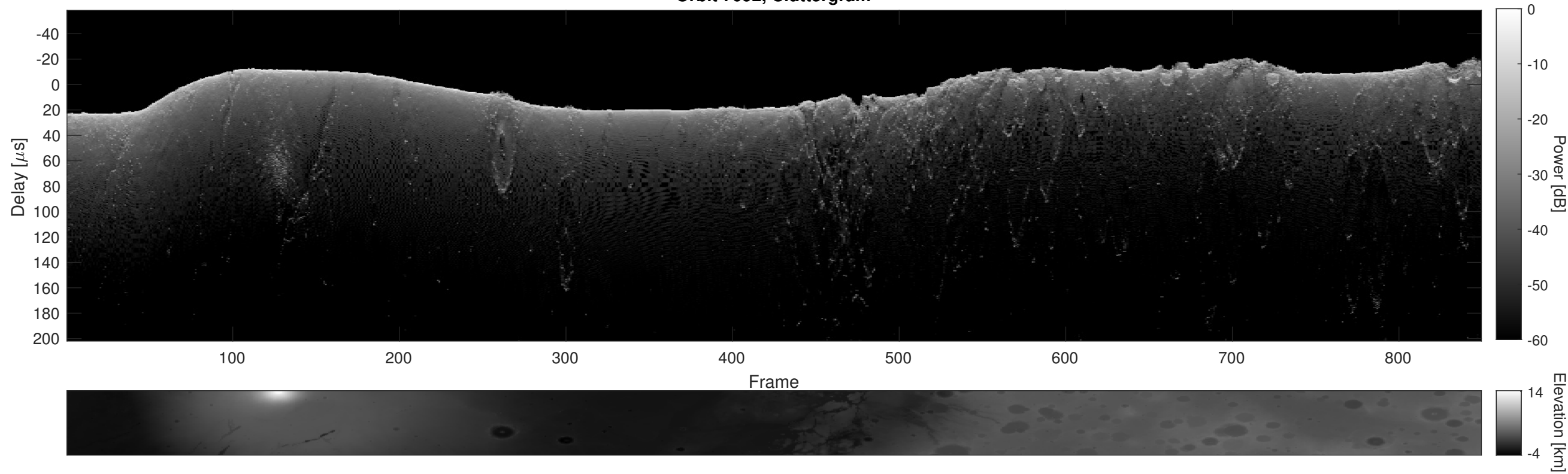
Orbit 7092, Cluttergram
