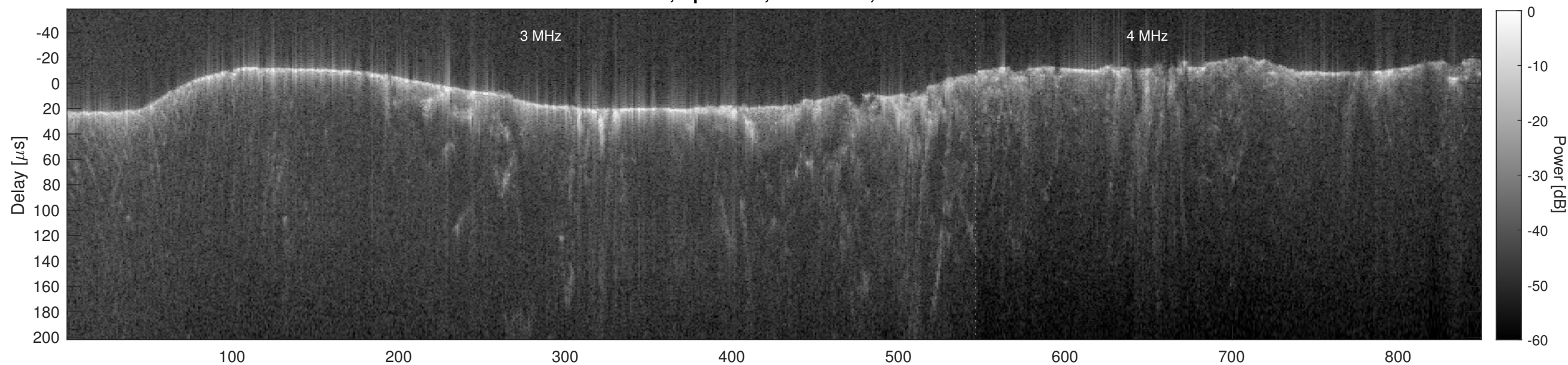
Orbit 7092, Cluttergram
